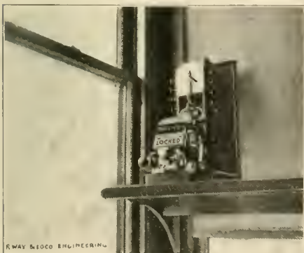
COLEMAN INSTRUMENT WITH CASING REMOVED SHOWING CARD, AND MINIATURE INDICATING SIGNAL.
